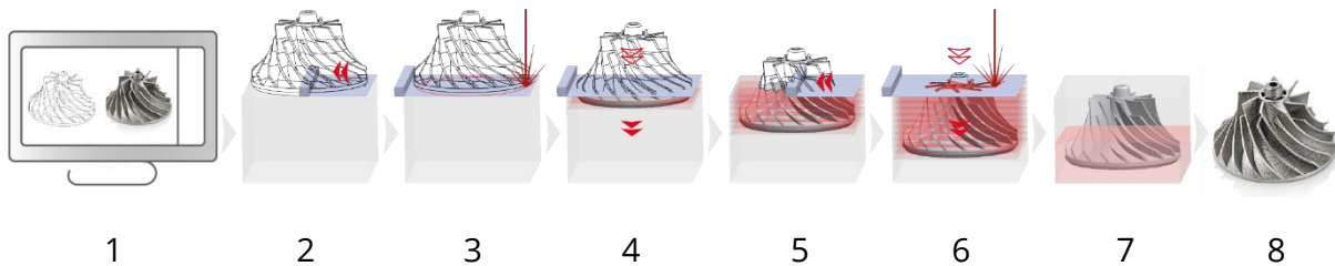
Figure 1: Scheme of the process steps for the manufacturing of laser sintered parts
